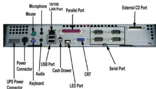
Main Board Interface Diagram
